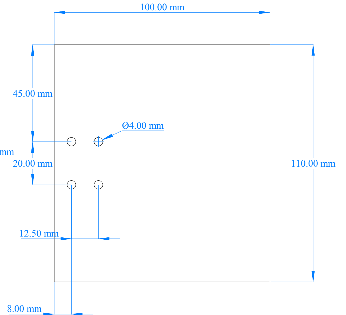
Camera Traveller Base Plate Drill to suit camera support
